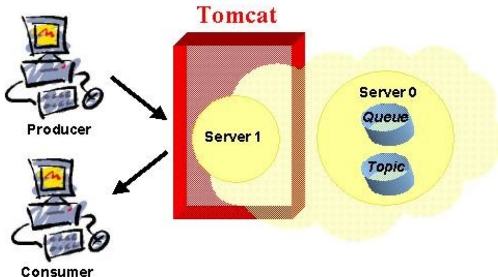
Figure 27 - SOAP sample configuration
