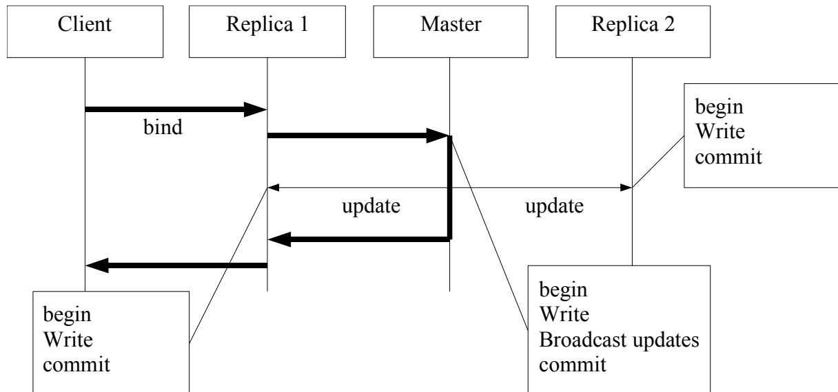
Figure 31 - Lazy propagation
