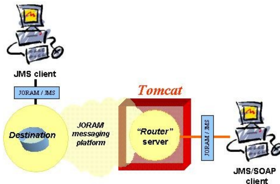
Figure 27 - A Joram platform providing a SOAP access
