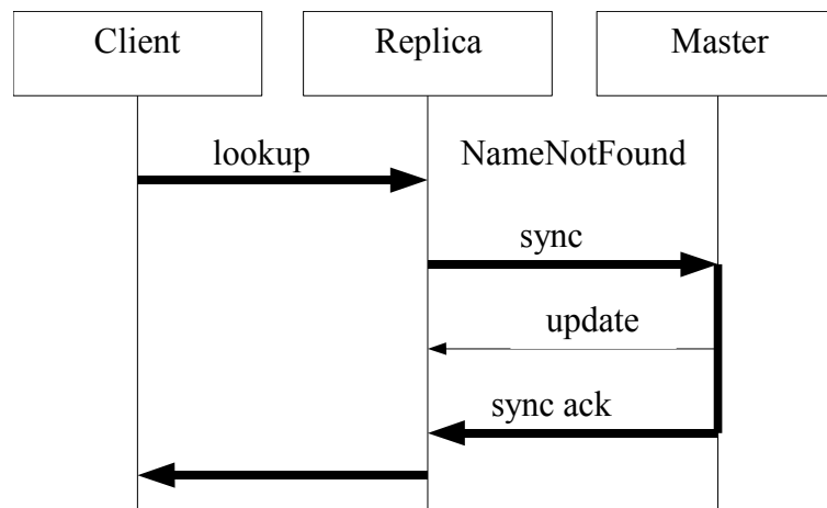
Figure 32 - Replicas synchronization
