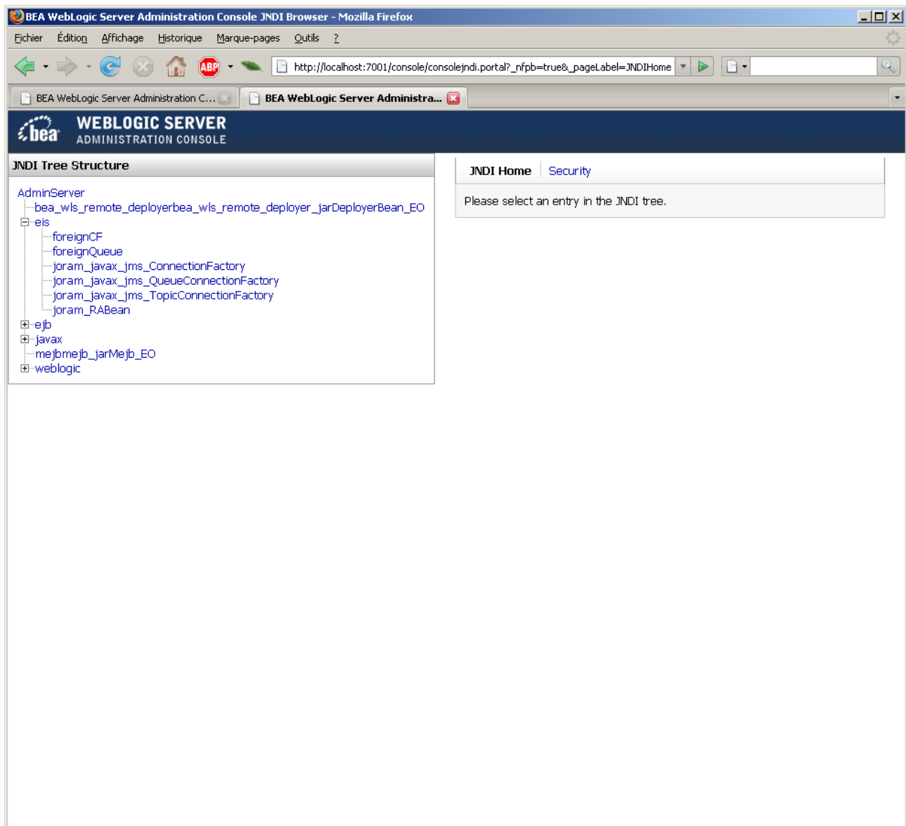
JNDI view
