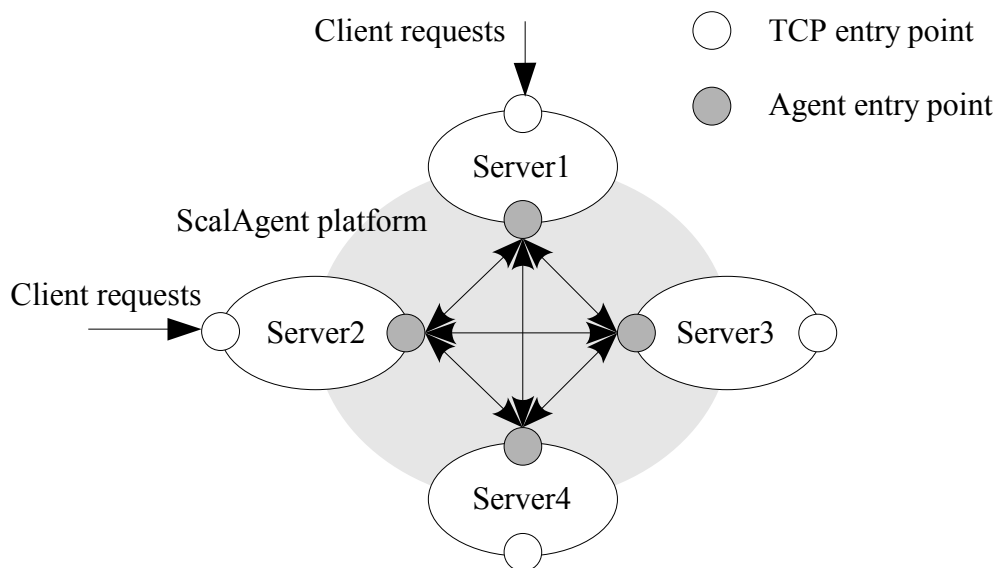
Figure 33 - Distributed configuration
