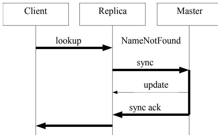
Figure 32 - Replicas synchronization
