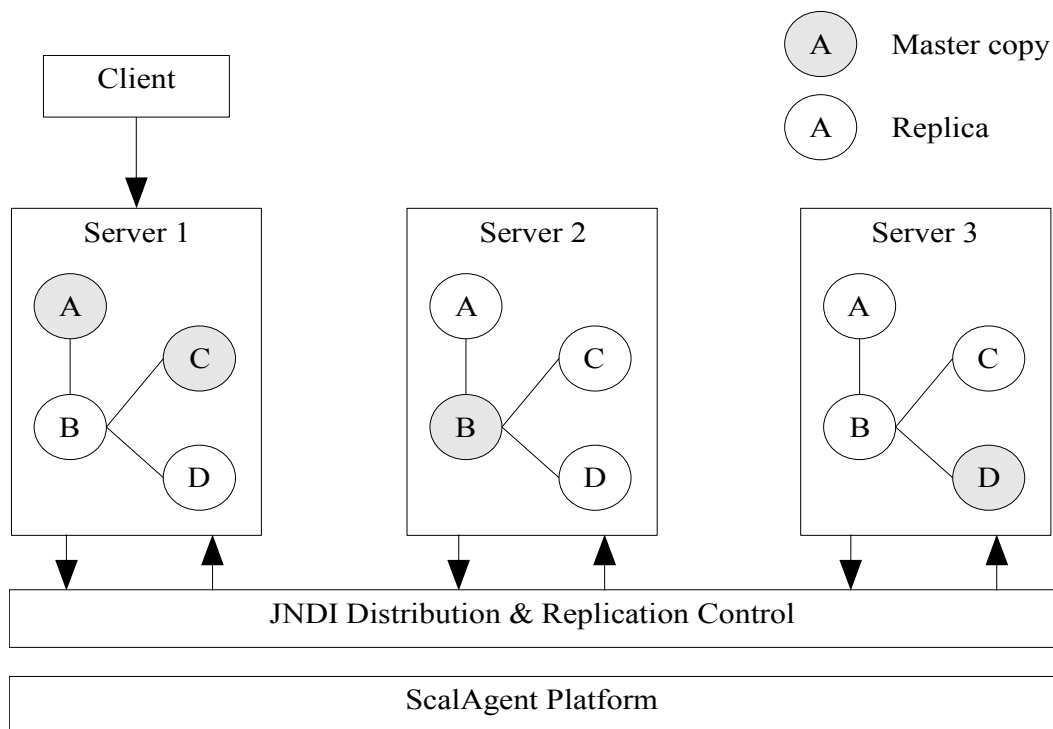
Figure 30 - JNDI replication
