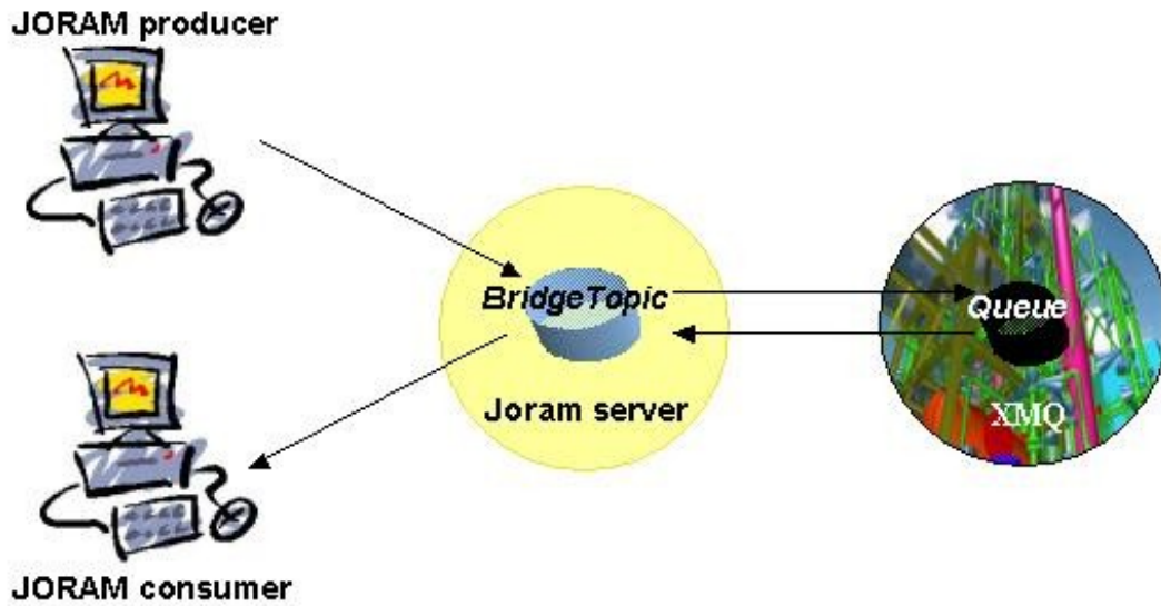
Figure 42 - Bridge sample
