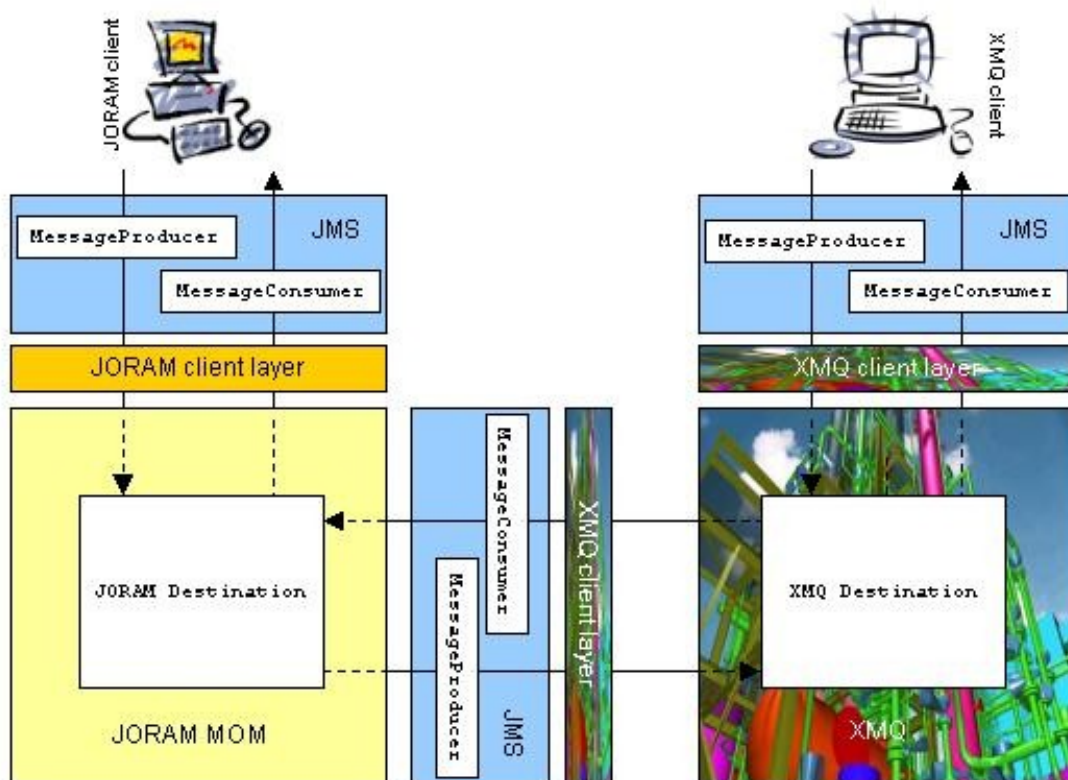
Figure 32 - Bridge communication diagram
