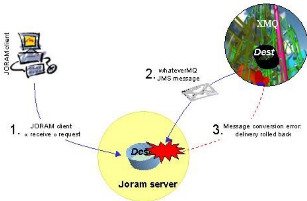
Figure 33 - Delivery rolled back by the JORAM bridge destination
