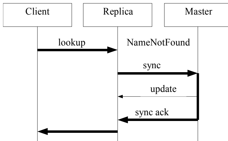
Figure 26 - Replicas synchronization
