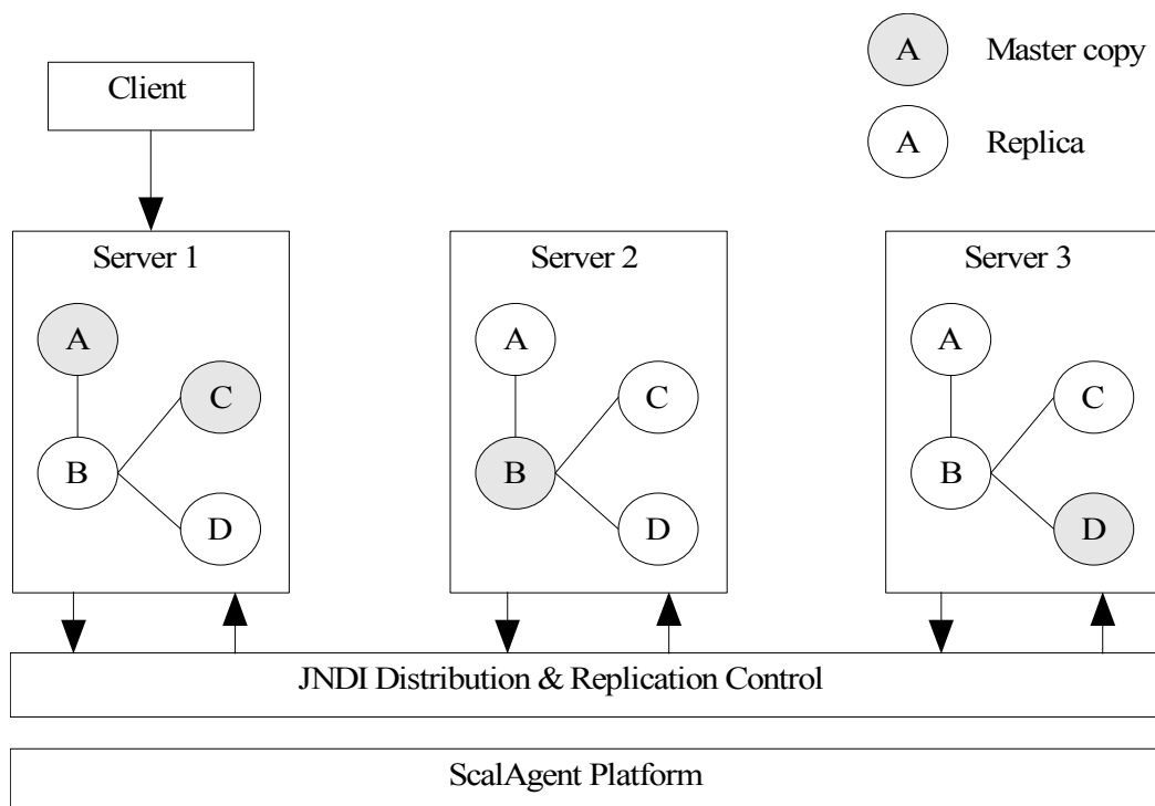
Figure 24 - JNDI replication
