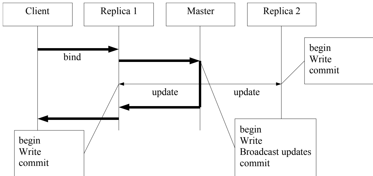
Figure 25 - Lazy propagation
