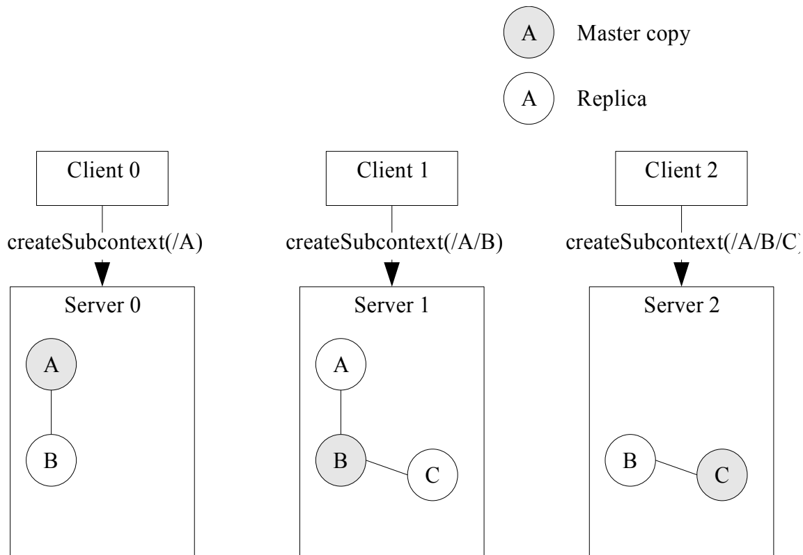
Figure 30 - The 3 servers configuration replicas
