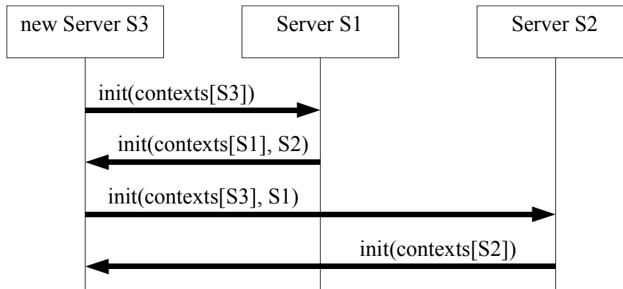
Figure 28 - Adding a new server
