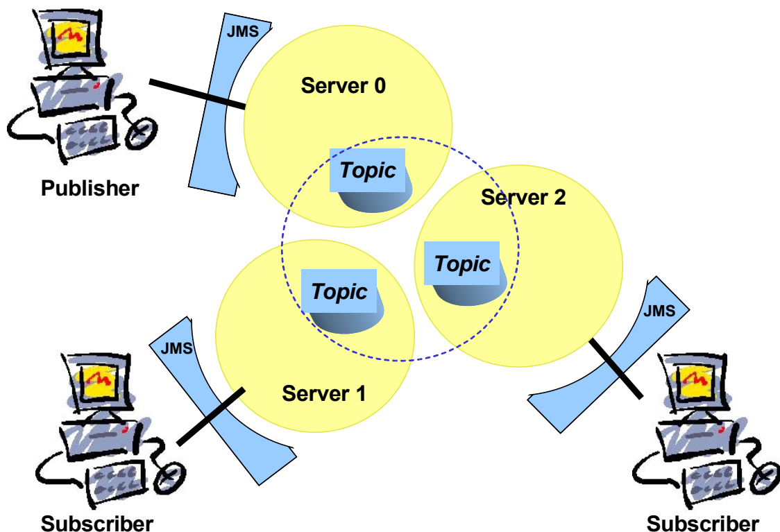
Figure 19 - Cluster sample configuration
