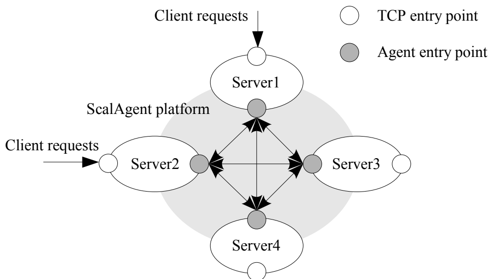
Figure 27 - Distributed configuration
