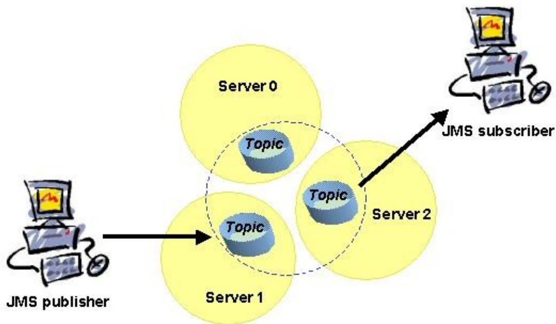
Figure 18 - A clustered topic
