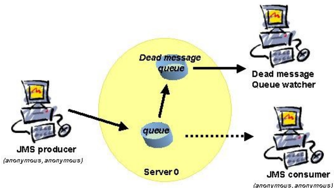
Figure 14 - Dead message queue sample
