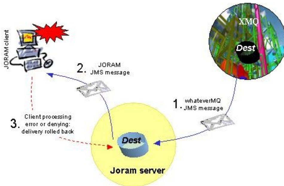
Figure 34 - Delivery rolled back by the JORAM client application
