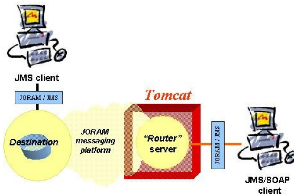
Figure 22 - A Joram platform providing a SOAP access
