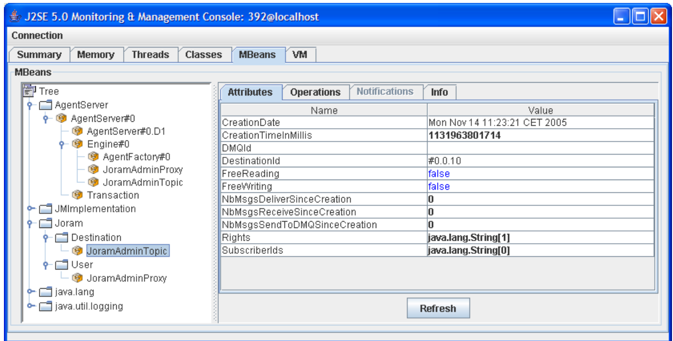
Figure 13 - JConsole view
