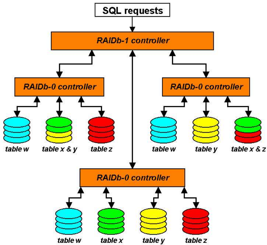
Figure 6. RAIDb-1-0 example
