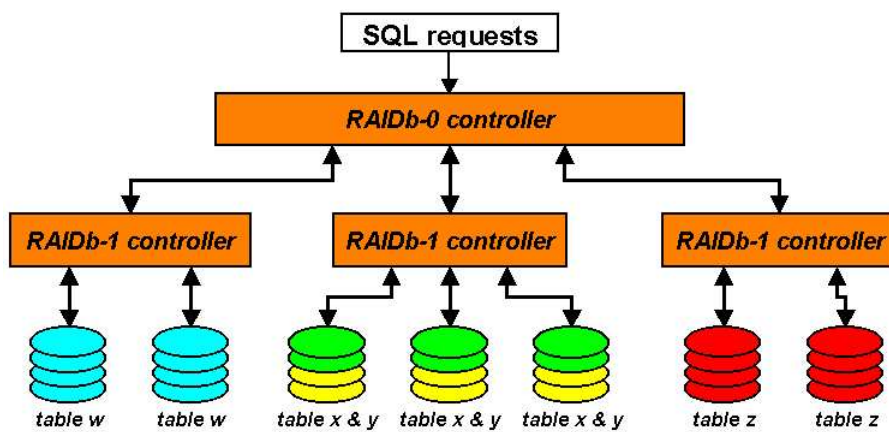
Figure 7. RAIDb-0-1 example
