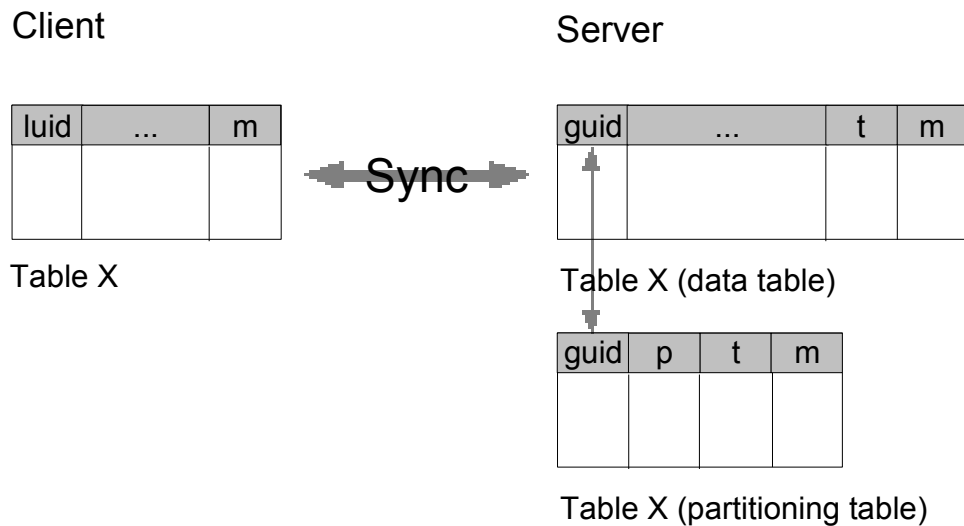
Figure 10 - Partitioned table scenario
