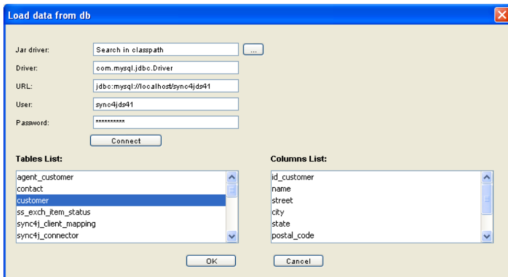
Figure 13 - Panel to load the fields from the database
