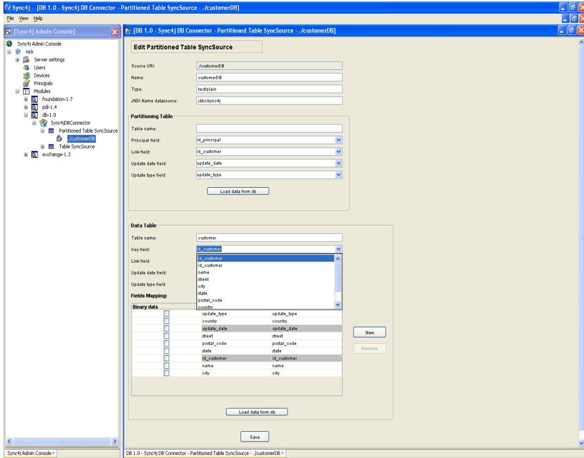
Figure 14 - The configuration panel after loading the data from database
