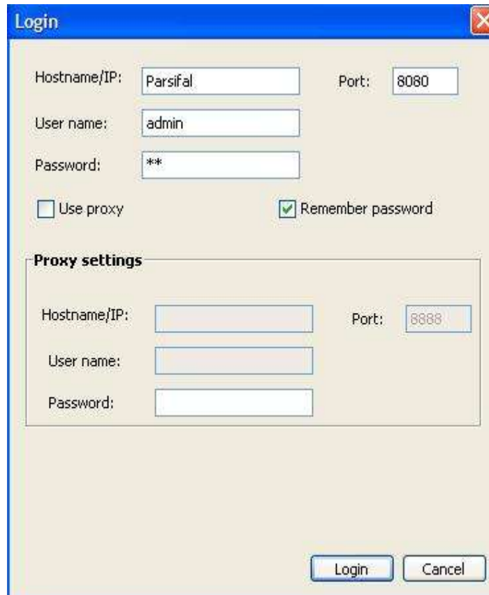
Figure 4 - Login Panel
